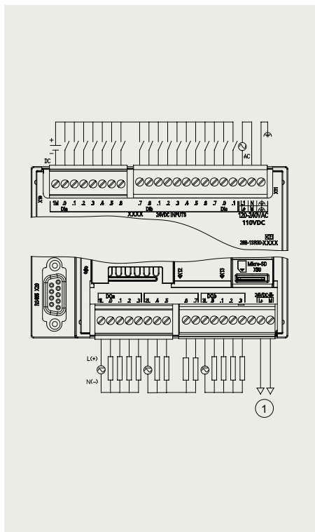
CPU SR30
