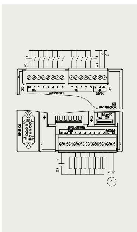
CPU ST20
