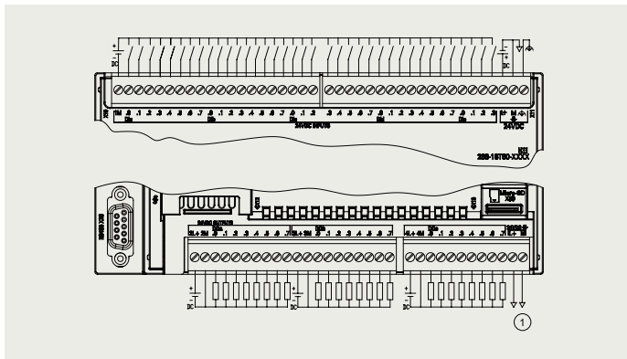
CPU ST60
