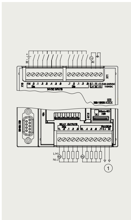
CPU SR20
